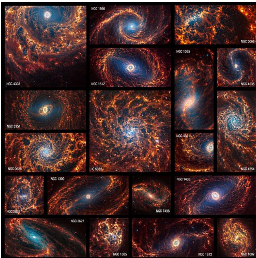
19 face-on spiral galaxies from the James Webb Space Telescope in near- and mid-infrared light. Older stars
