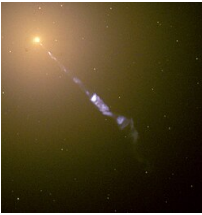
A jet of particles is being emitted from the core of the elliptical radio galaxy M87 .
