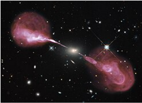
Hercules A , supergiant elliptical radio galaxy
